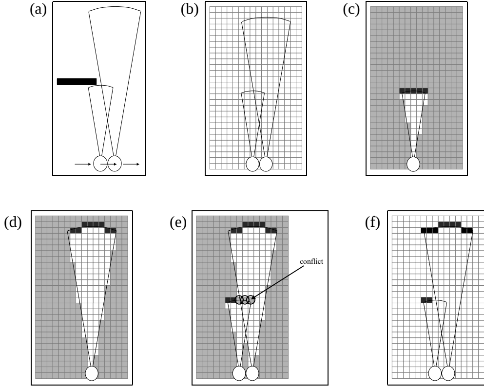
Figure 2: The problem with current occupancy grid mapping algorithms: For the environment shown in Figure (a), a passing robot might receive the (noise-free) measurement shown in (b). Inverse sensor models map these beams into probabilistic maps. This is done separately for each grid cell and each beam, as shown in (c) and (d). Combining both interpretations may yield a map as shown in (e). Obviously, there is a conflict in the overlap region, indicated by the circles in (e). The interesting insight is: There exist maps, such as the one in diagram (f), which perfectly explain the sensor measurement without any such conflict. For a sensor reading to be explained, it suffices to assume an obstacle somewhere in the cone of a measurement, and not everywhere. This effect is captured by the forward models described in this article.
